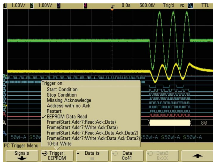
Figure 12. Triggering on a 3-cycle chirp with I 2 C triggering and decode in an Agilent MSO.
