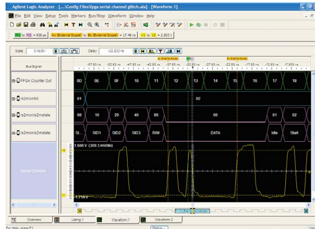
Figure 14. A time-correlated display of an oscilloscope's waveforms ported into a logic analyzer's display.
