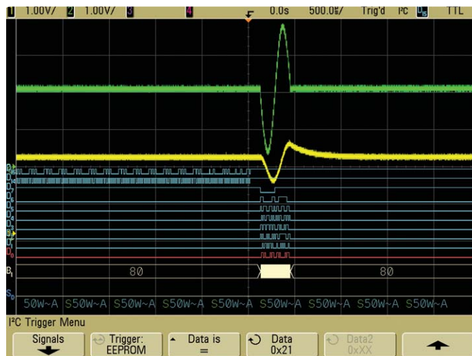
Figure 13. Triggering on a 1-cycle chirp with I 2 C triggering and decode in an Agilent MSO.
