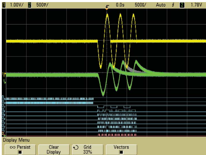
Figure 11. Conventional oscilloscope edge triggering fails to synchronize on specific-length chirps.
