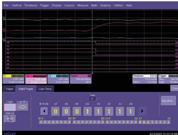
Figure 4. Without time-qualification, the scope triggers on unstable/transitional states (LeCroy WaveRunner with MSO option).
