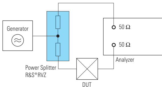
Test setup for transmission measurements
