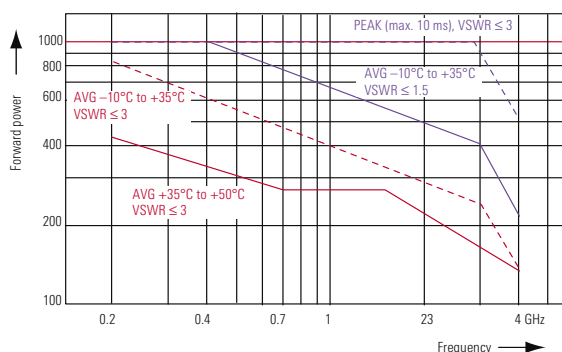
Power-handling capacity
