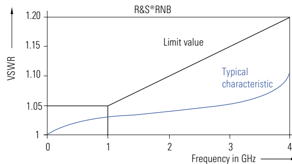
Limit value and typical VSWR characteristics of the R&S®RNB
