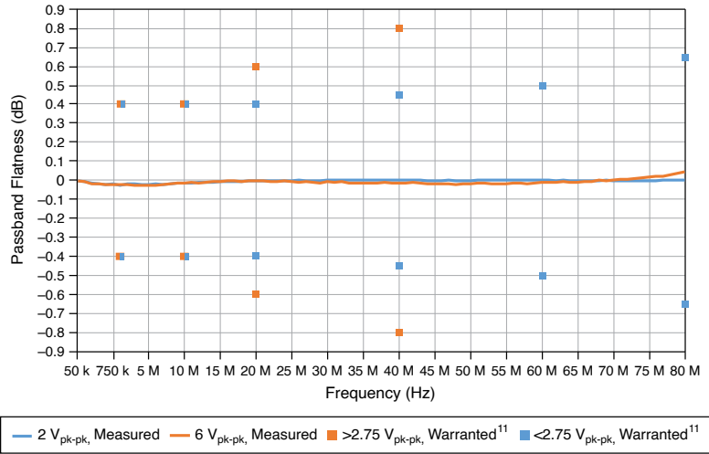
Figure 1. Passband Flatness
