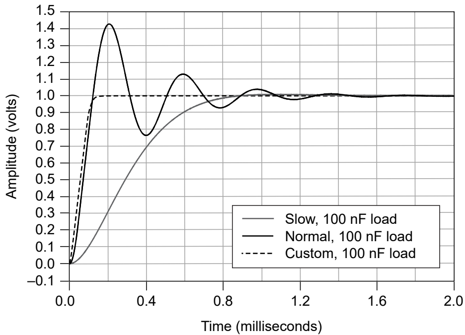
Figure 8. 1 mA Range, 100 nF Load Step Response, Typical
