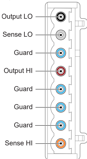
Figure 1. PXIe-4139 Connector Pinout
