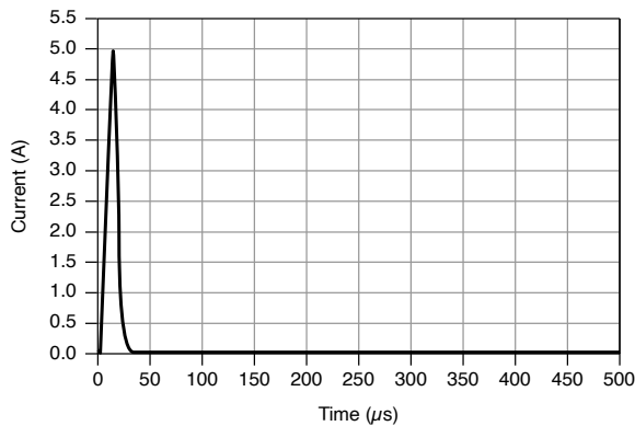
Figure 13. 10 \mu s Pulse Output with Load, Custom Transient Response
