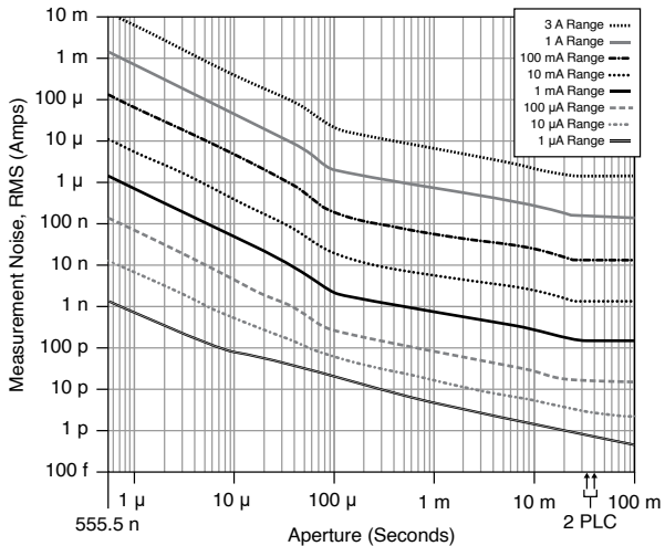
Figure 5. Current Measurement Noise vs. Measurement Aperture, Nominal
