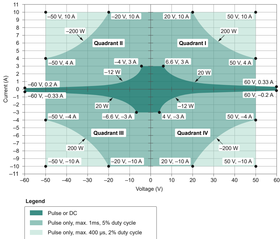
Figure 3. Quadrant Diagram for PXIe-4139 (20W)
