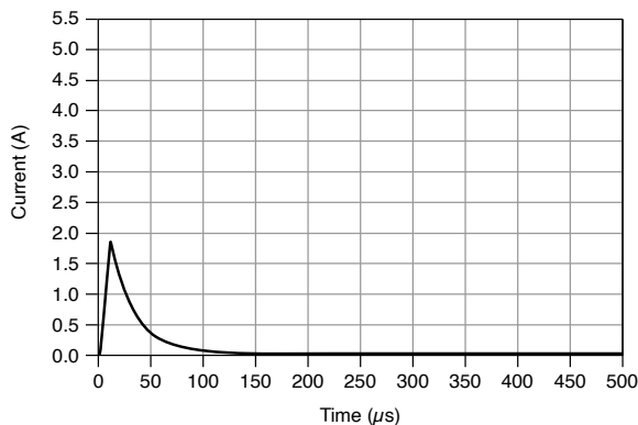
Figure 12. 10 \mu\text{s} Pulse Output with Load, Fast Transient Response
