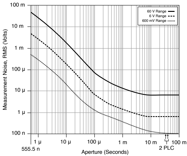
Figure 4. Voltage Measurement Noise vs. Measurement Aperture, Nominal
