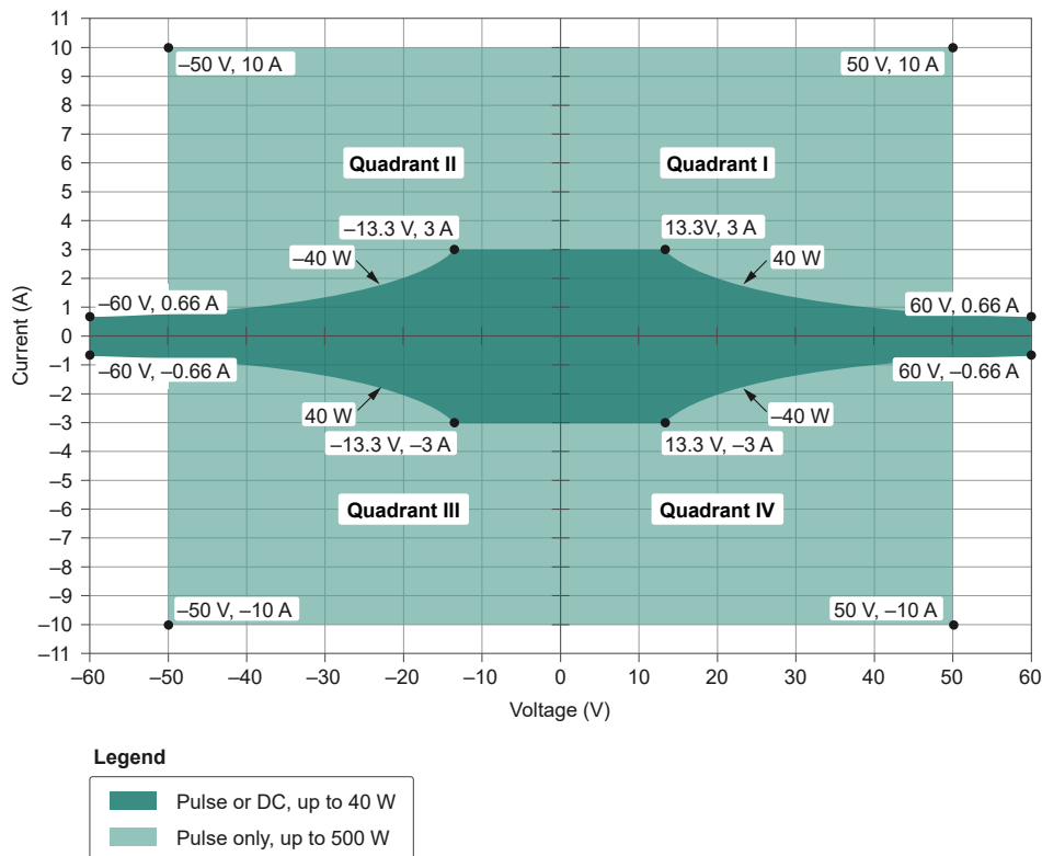
Figure 2. Quadrant Diagram for PXIe-4139 (40W)
