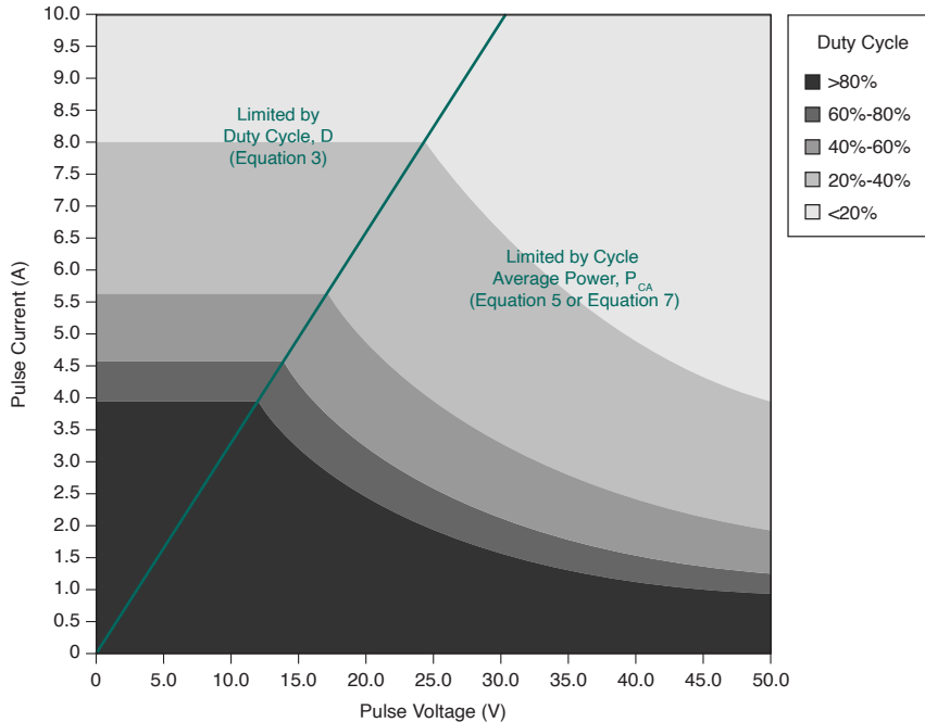
Figure 9. Duty Cycle vs Pulse Current and Pulse Voltage
