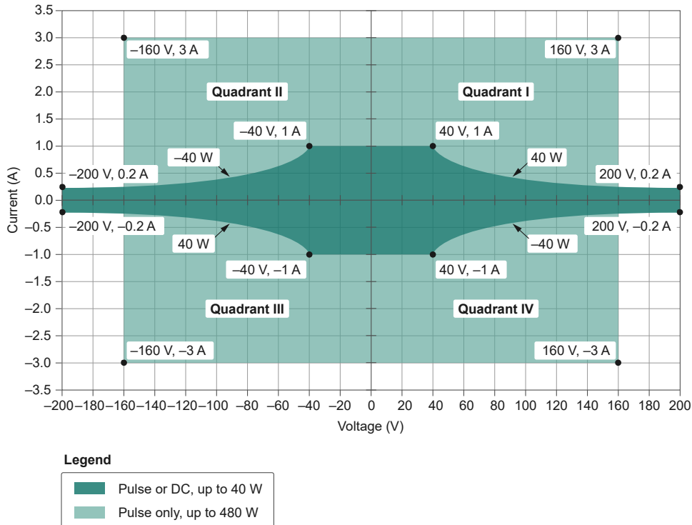
Figure 1. Quadrant Diagram for PXIe-4135 (40W)
