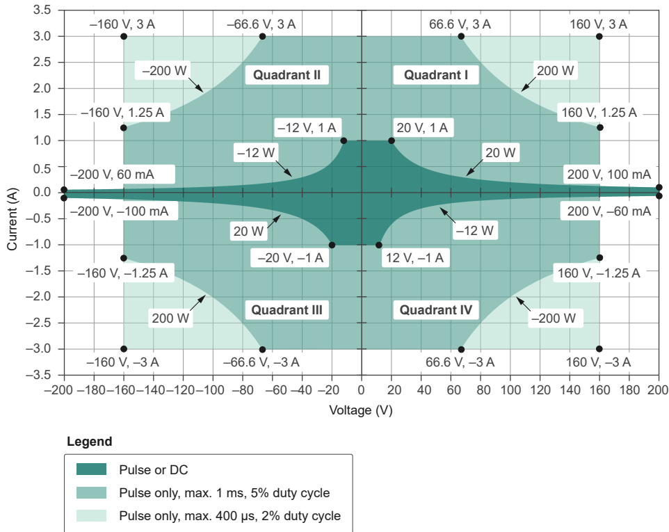
Figure 2. Quadrant Diagram for PXIe-4135 (20W)
