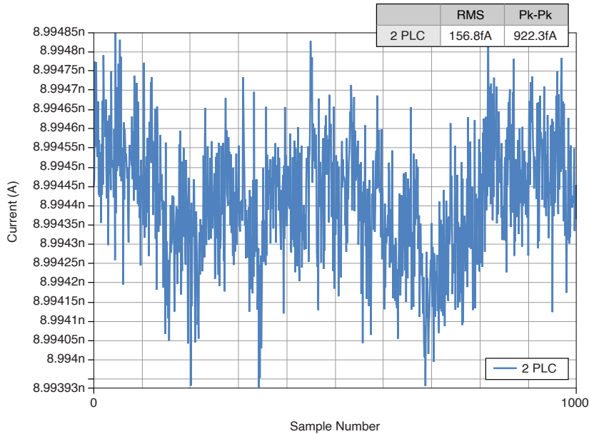
Figure 6. Measurement Noise, 10 nA Range, 1 G \Omega Load, 9 V, 3 m Cables, Nominal
