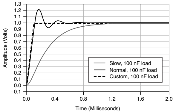
Figure 12. 1 mA Range, 100 nF Load Step Response, Nominal
