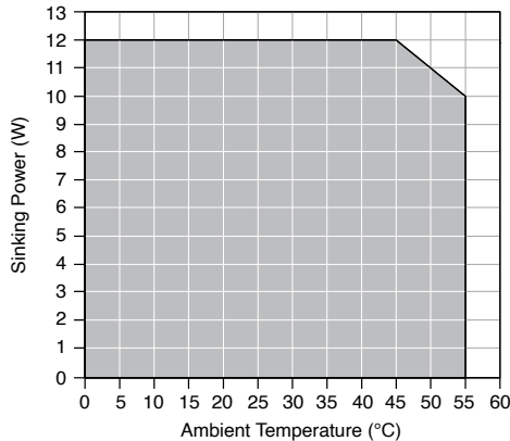
Figure 7. Sinking Power vs. Ambient Temperature Derating
