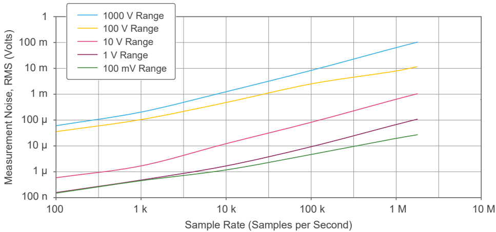
Figure 5. PXIe-4081 Voltage Waveform Noise with Input Shorted, Typical
