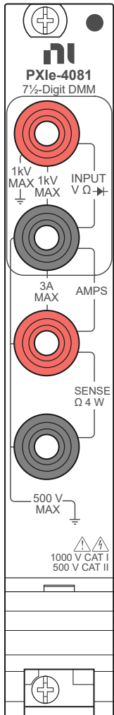
Figure 1. PXIe-4081 Connector Pinout
