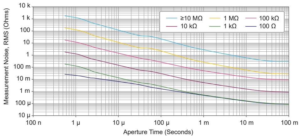
Figure 3. PXIe-4081 Resistance Noise, Typical
