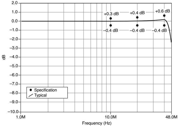
Figure 2. Pulse Response, Low-Gain Amplifier Path 50 Ω Load
