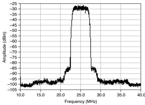
Figure 12. W-CDMA Physical Layer [59][57] Internal (High Resolution) Sample Clocking = 92.16 MHz
