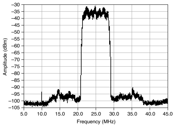
Figure 14. DVB Physical Layer [60][62][57] Internal (High Resolution) Sample Clocking = 96.88 MHz
