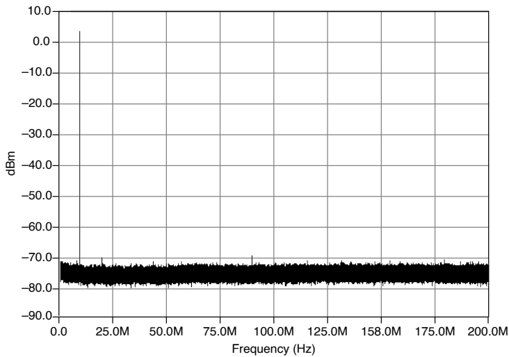
Figure 5. 10 MHz Single-Tone Spectrum [22] , Low-Gain Amplifier Path, 100 MS/s, DAC Interpolation
