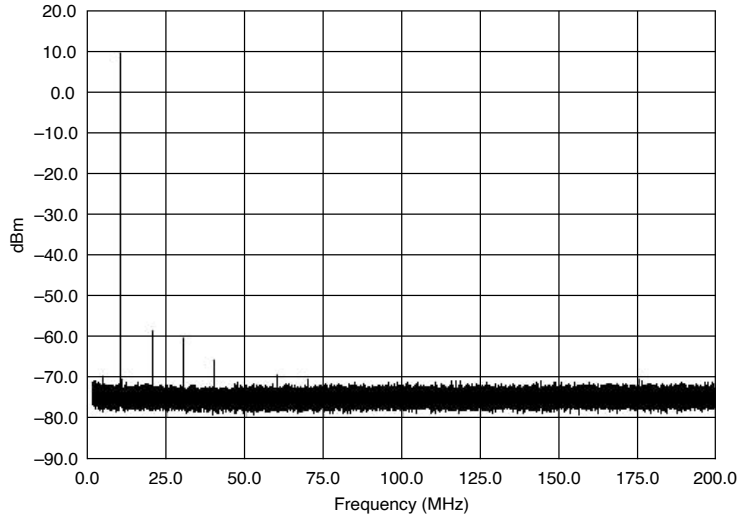
Figure 6. Direct Path, Two-Tone Spectrum [22] , Typical
