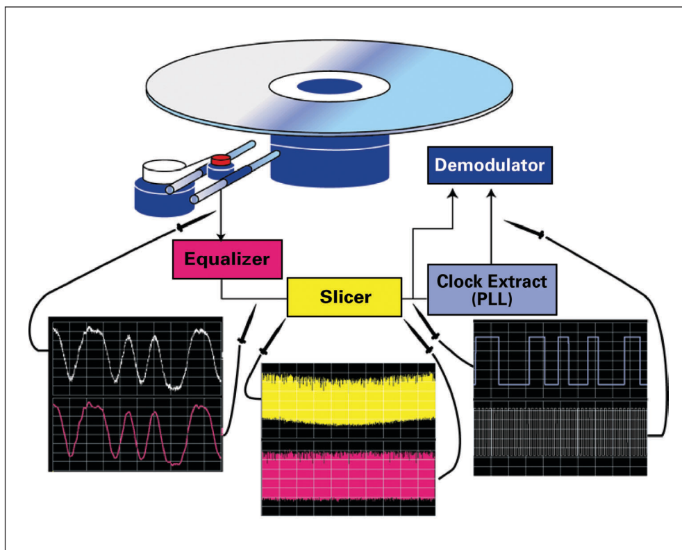
This figure depicts a block diagram of signal processing in optical disk drive. AORM software extracts baseline fluctuation and slices the RF signal to generate a binary signal. Then the software PLL extracts clock content from the incoming binary signal, and the decoder decodes from binary signal timing referred to the clock.
