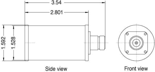
Type N Female
