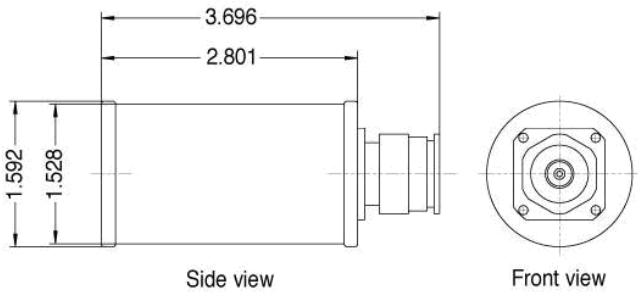
Type N Male
