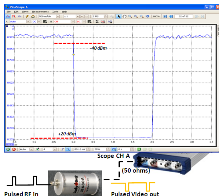
Measuring Option 0W2 Wideband, Negative Detector, Analog Video Output Signal
