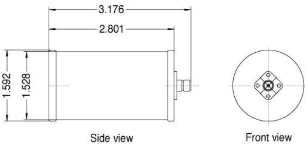
SMA Female
