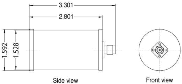
SMA Male
