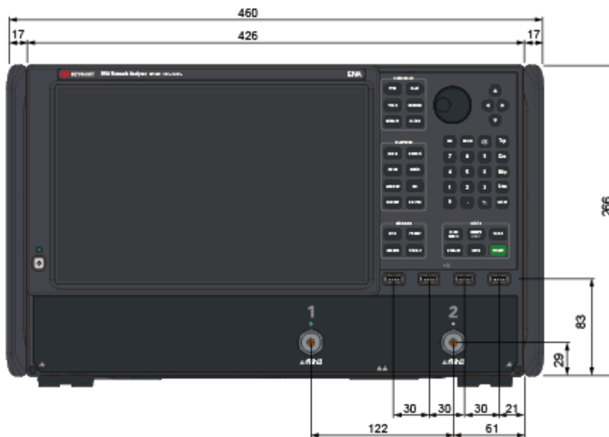
Dimensions (front view, E5080B with option 2D0/2K0/2L0 (3.5 mm), in millimeters)
