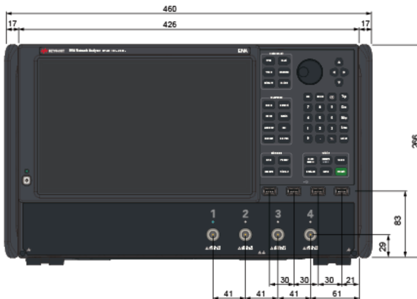
Dimensions (front view, E5080B with option 440/460/490/442/462/492 (Type-N), in millimeters)
