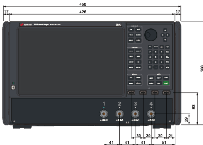
Dimensions (front view, E5080B with option 4D0/4K0/4L0/4D2/4K2/4L2 (3.5 mm), in millimeters)
