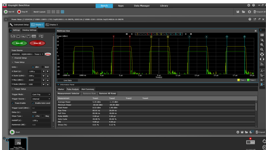
Figure 9. Multi-channel trace display with 4-pairs of gates and automatic pulse parameters measurement (sample screen shot with two U2042XAs).
