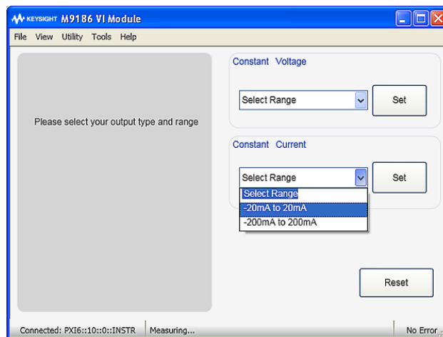
Figure 3. Module configuration - constant current.
