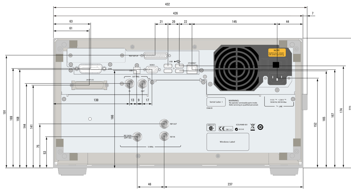
Figure 22. Dimensions (rear view, in millimeters)
