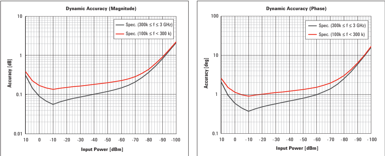
Figure 18. Option 115, 135, 117, 137, 215, 235, 217, 237
