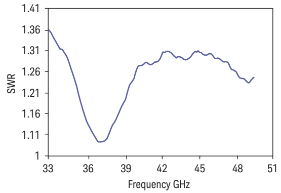
Typical SWR, 33 to 50 GHz (25 ± 10 °C) for N8486AQ power sensor
