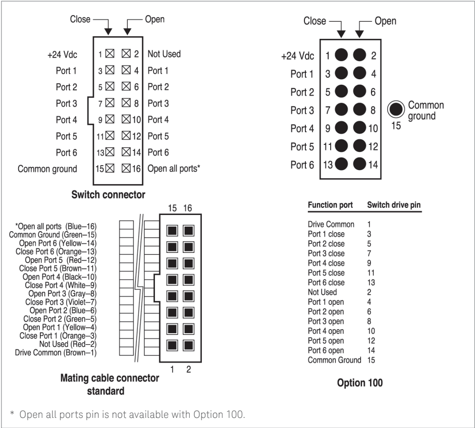
Figure 7. Drive connection diagrams
