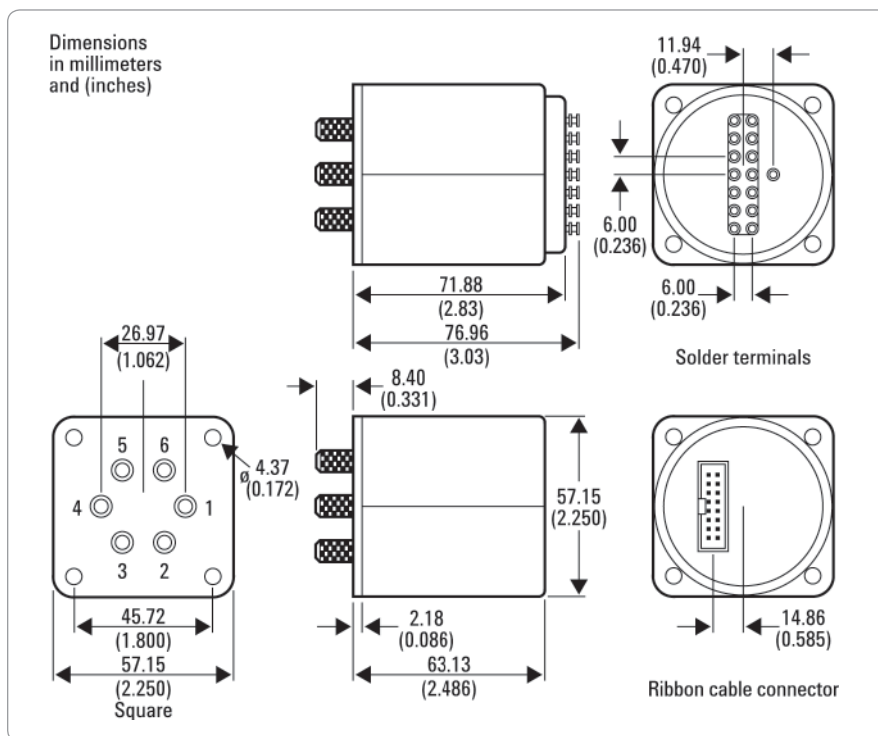
Figure 7. Product outline
