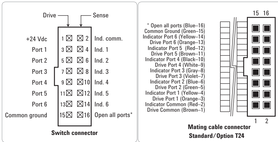
Figure 6. J1 connector configuration
