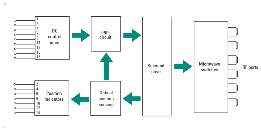
Figure 4. Agilent 87406B block diagram
