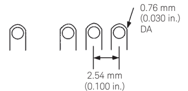
Figure 1b. Suggested receptacle dimensions
