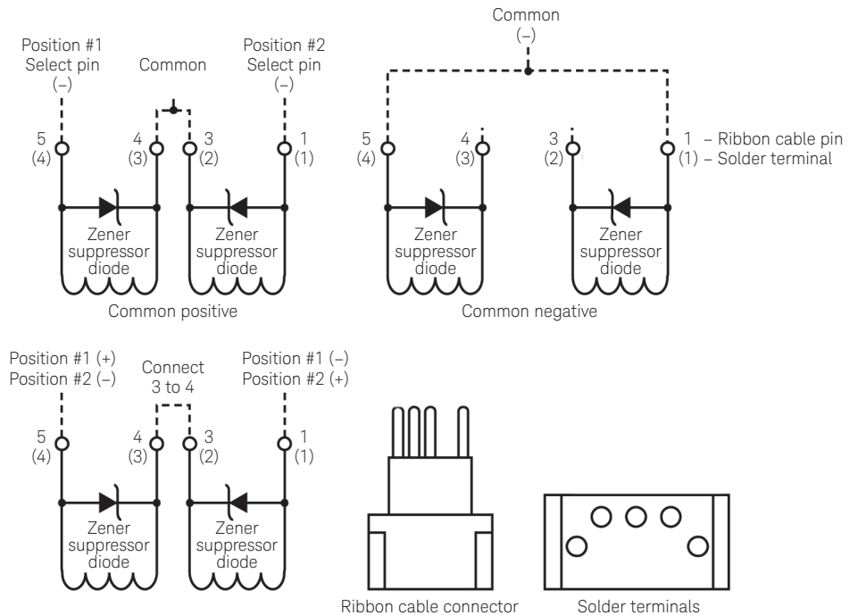
Figure 1a. DC control circuit configurations
