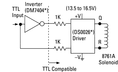
Figure 5. Typical 8761A driver circuit
