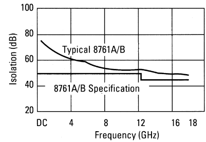
Figure 1. Typical port-to-port isolation
