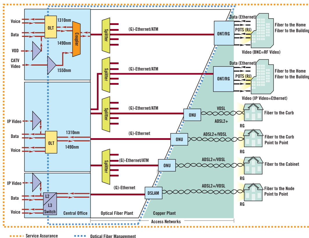
Figure 1 - FTTx Architectures
