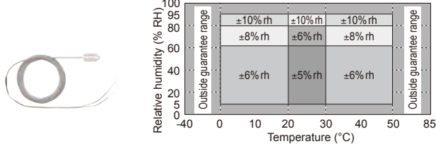
Humidity sensor Z2000 accuracy
