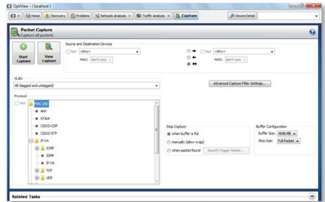
Packet capture
