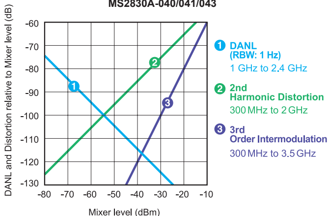
Distortion Characteristics (Spectrum Analyzer) MS2830A-040/041/043
