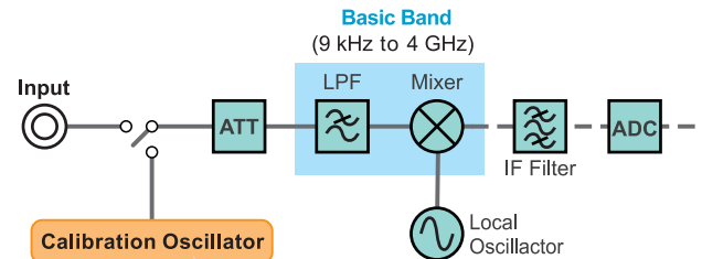
MS2830A Block Diagram
