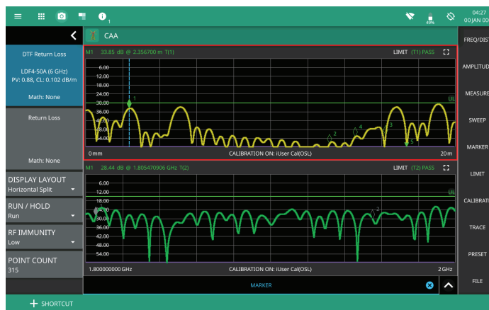
Split Screen Showing Return Loss and DTF Return Loss of a 20 Meter Cable Feed
