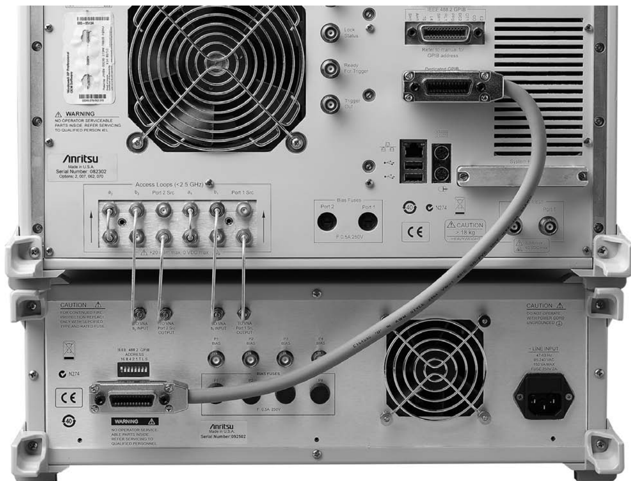
MN469xB Test Set Rear Panel and connections to base VNA.
