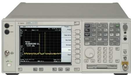
Agilent E4448A PSA signal analyzer
