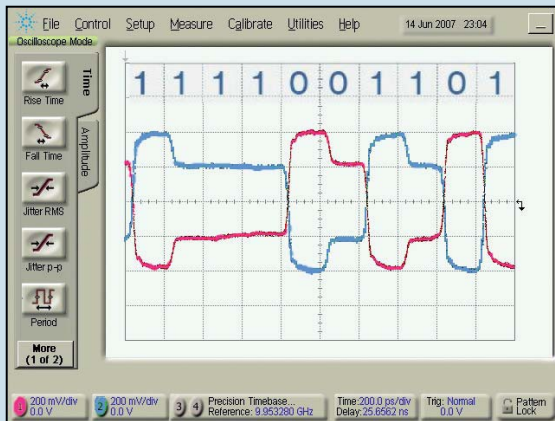
Figure 1: De-emphasized differential signal generated with the N4916A and the J-BERT N4903A/B at 5 Gb/s data rate with 6dB de-emphasis.
