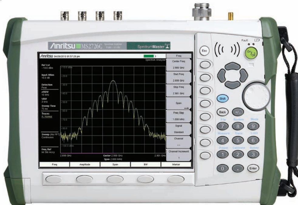
Spectrum Master™ MS2726C Spectrum Analyzer
