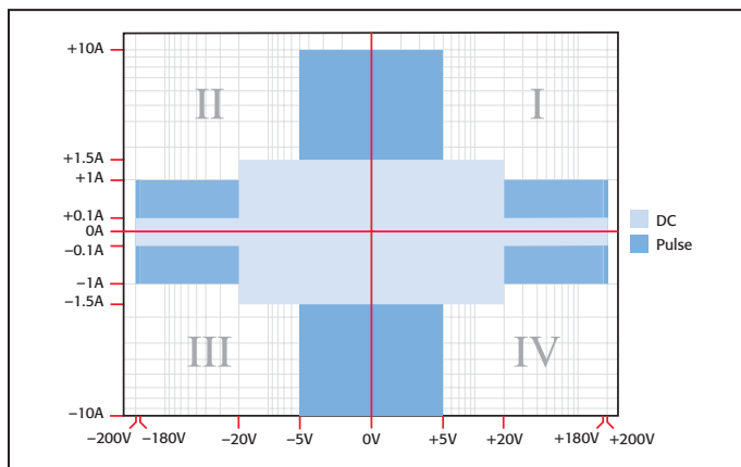
Models 2611A and 2612A I-V capability
