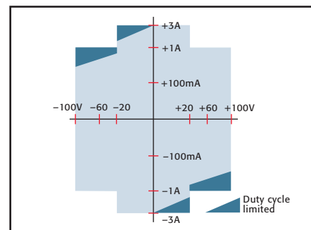
Model 2425 100W SourceMeter
