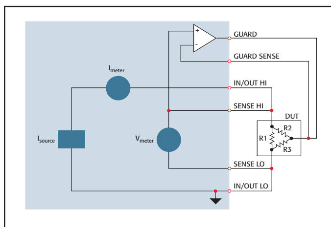
6-Wire Ohms Circuit. All test current flows through R1 because the high current guard drives the voltage across R2 to 0V.
