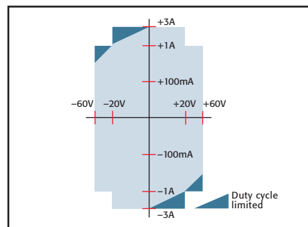
Model 2420 3A SourceMeter
