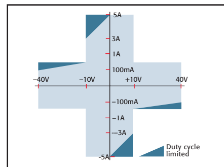
Model 2440 5A SourceMeter
