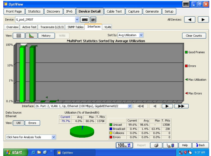
Multi-port statistics
