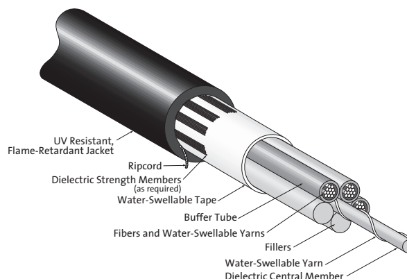
FREEDM Loose Tube Gel-Free Cable | Drawing ZA-1894
