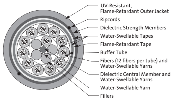
144-Fiber FREEDM Loose Tube Gel-Free Cable | Drawing ZA-511
