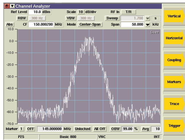
Spectrum Analyzer
